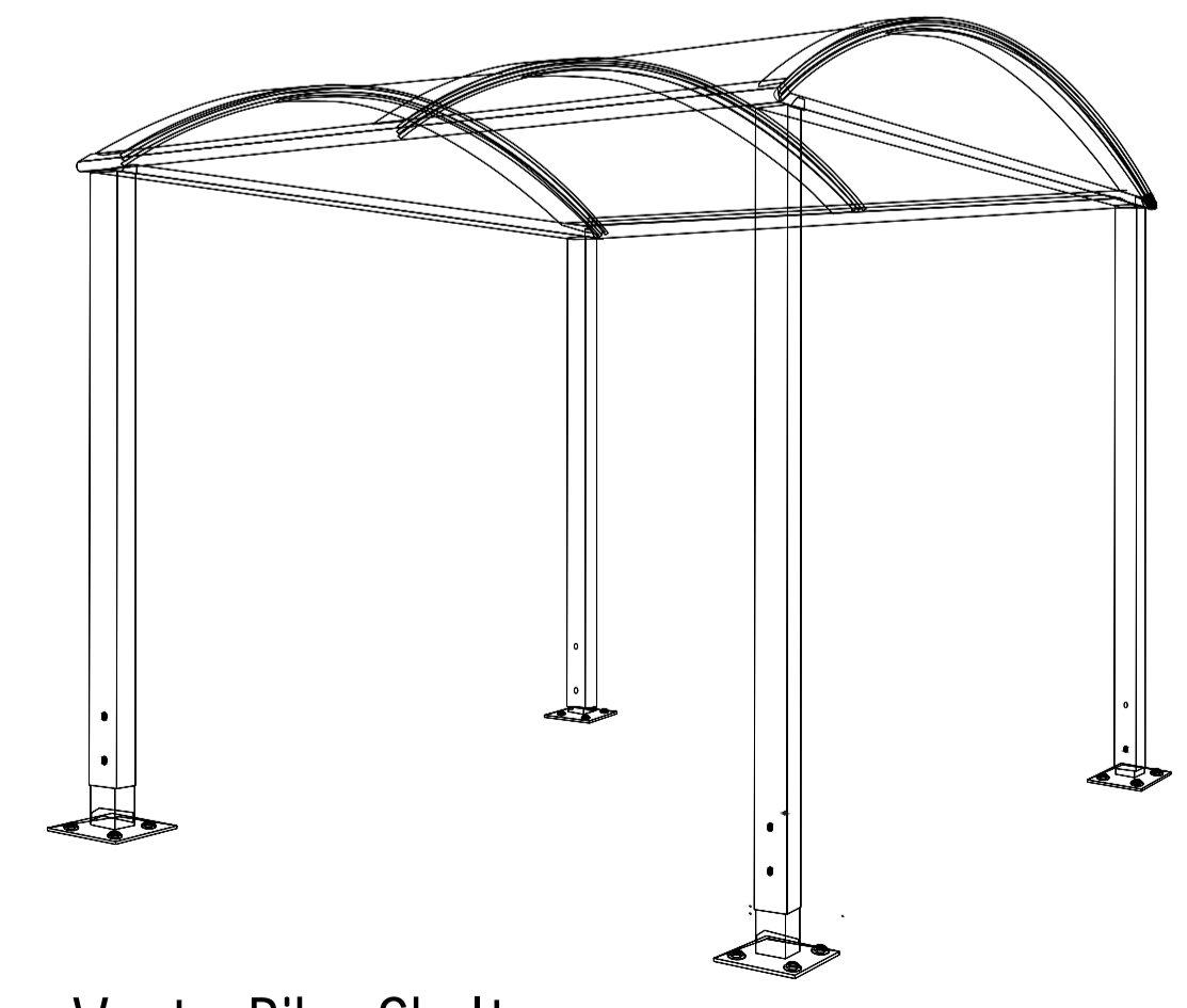
Voute Bike Shelter
