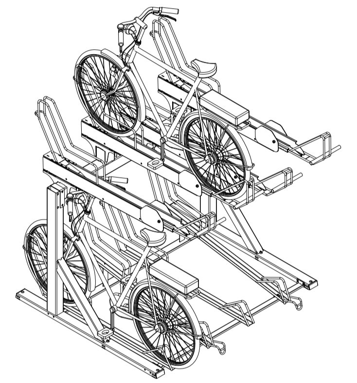
Velo Up Regular Two Tier Bike Storage
