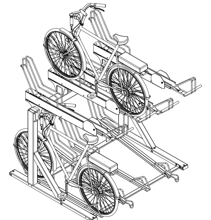
Velo Up Regular Two Tier Bike Storage
